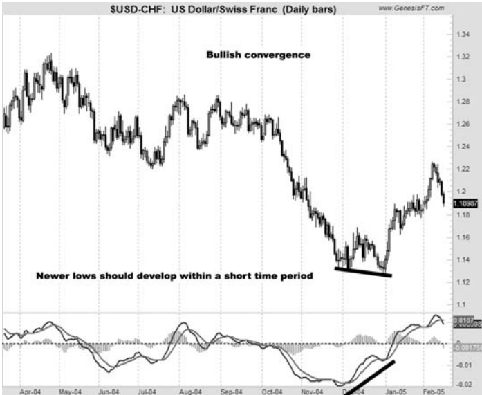
FIGURE 5.8 MACD Bullish Convergence Shows in Moving Average Component Used with permission of GenesisFT.com.
